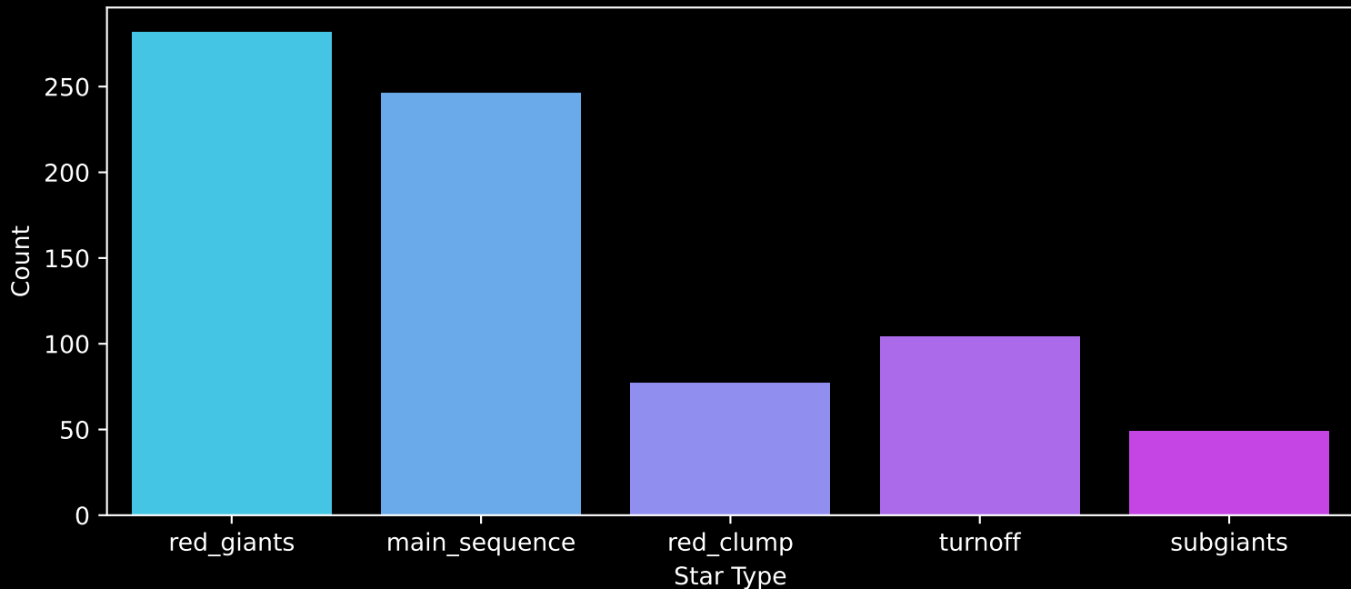
APOGEE DR17 Field: [K04_083+13] Count plot of Star Type
