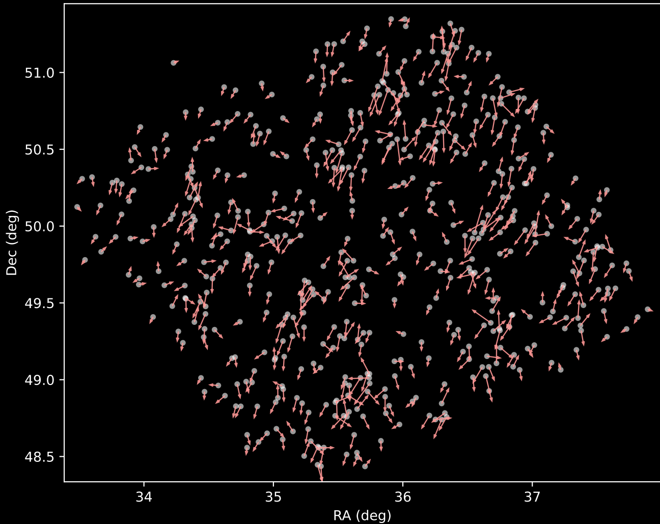
APOGEE DR17 Cluster 7 Proper Motion Vectors (n=528)
