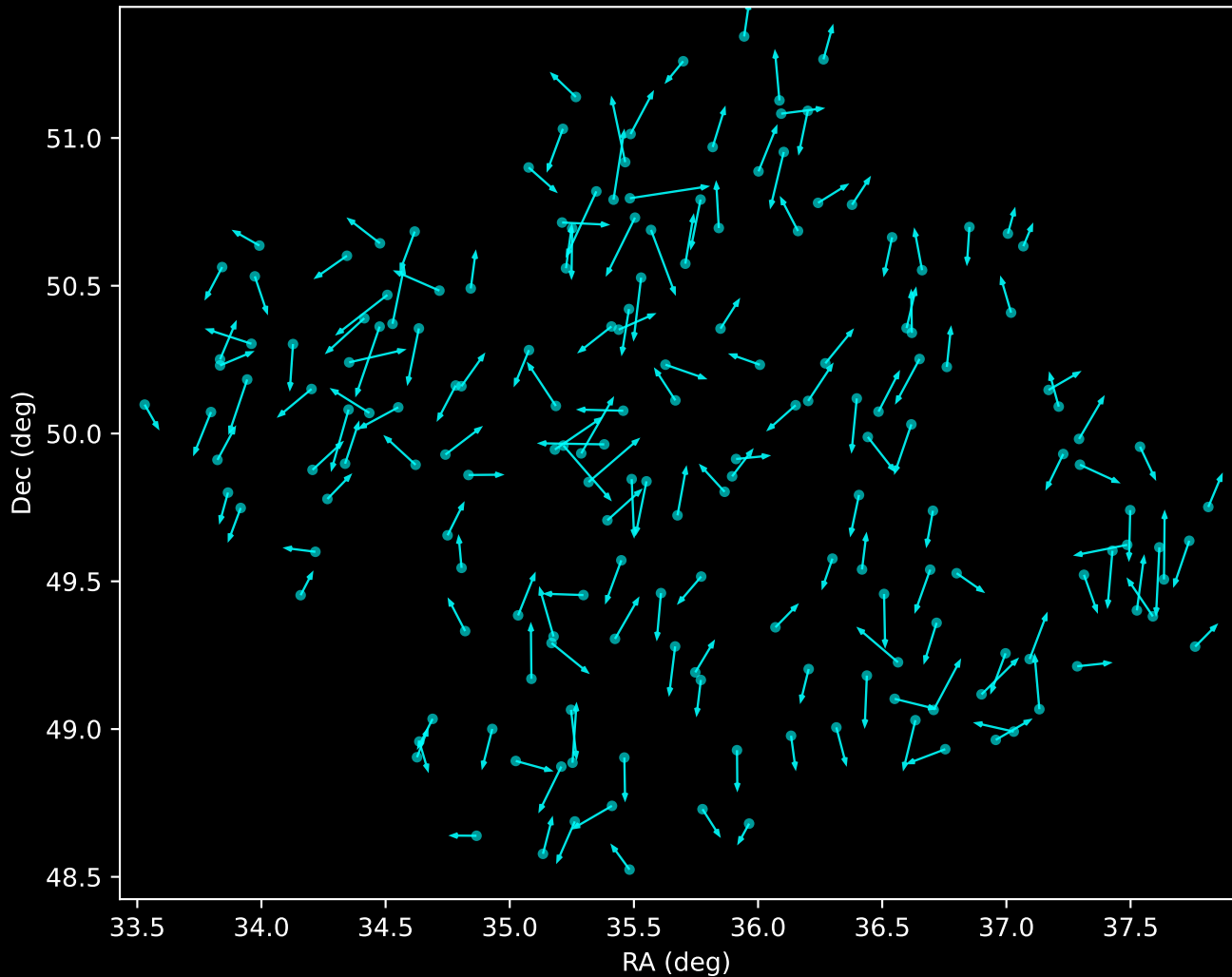
APOGEE DR17 Noise Stream Proper Motion Vectors (n=180)
