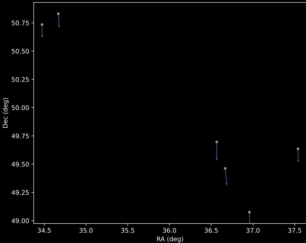
APOGEE DR17 Cluster 8 Proper Motion Vectors (n=6)
