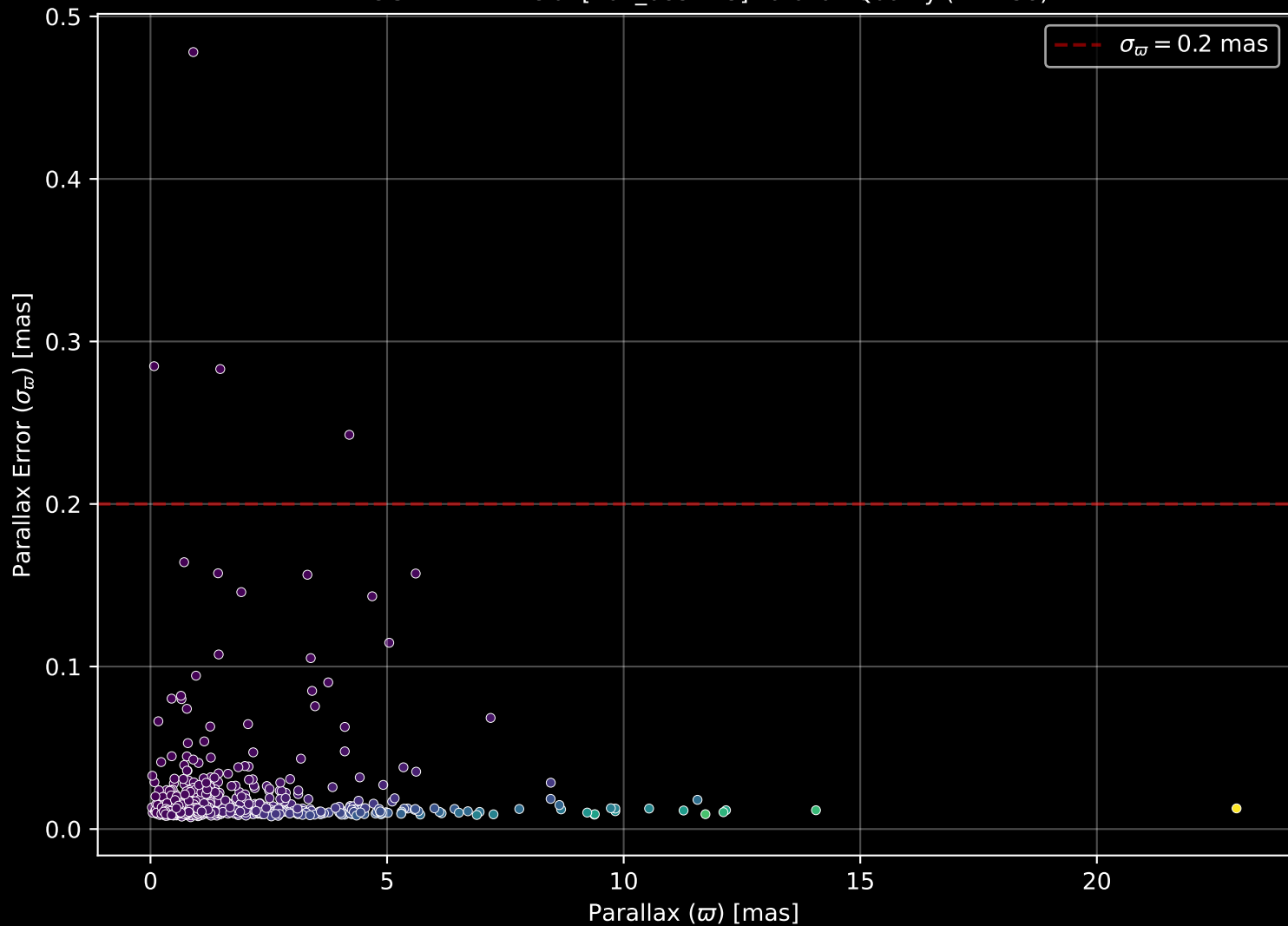
APOGEE DR17 Field: [K04_083+13] Parallax Quality (n= 758)
