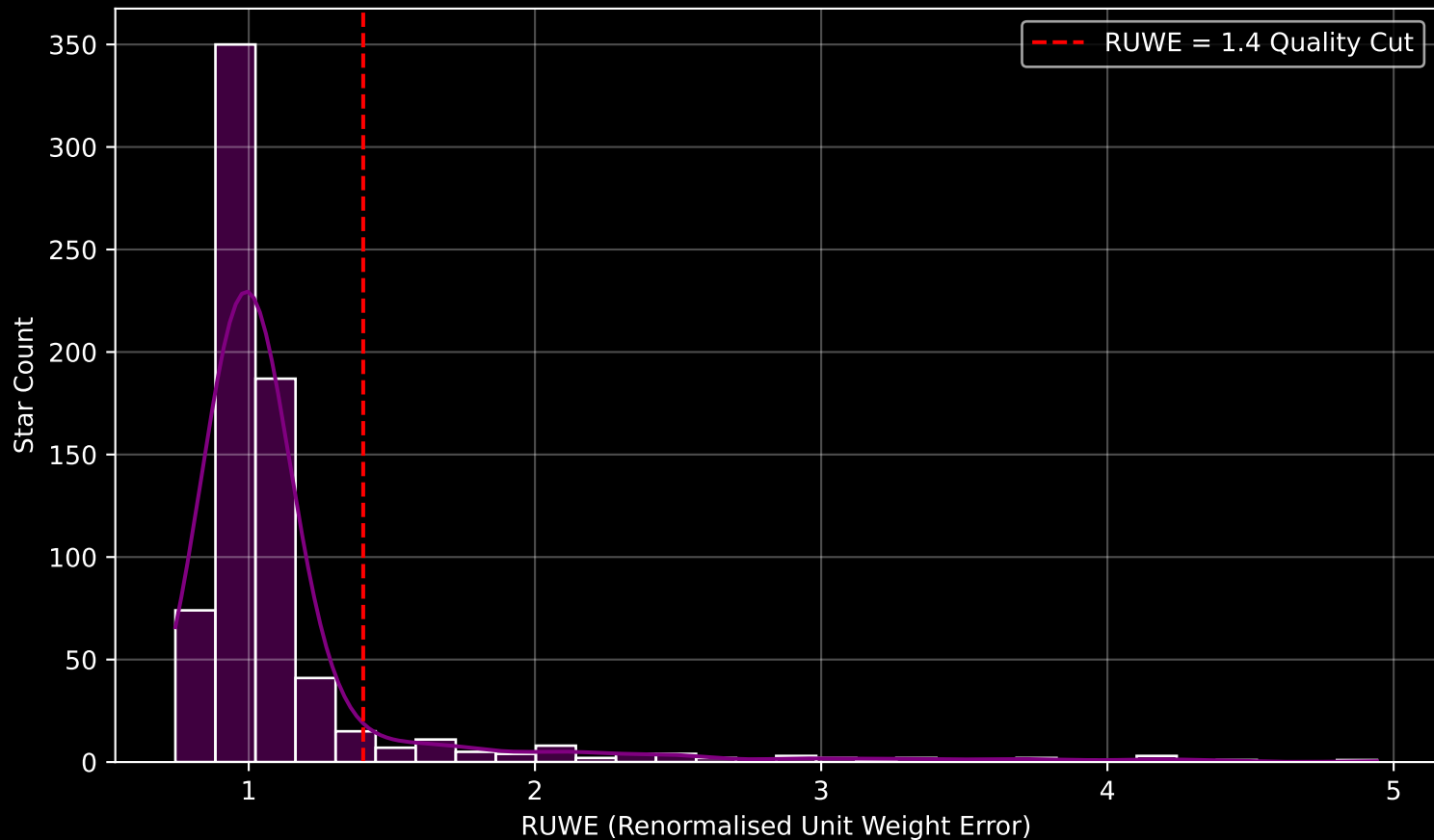
GAPOGEE DR17 Field [K04_083+13] RUWE Distribution (n= 732)
