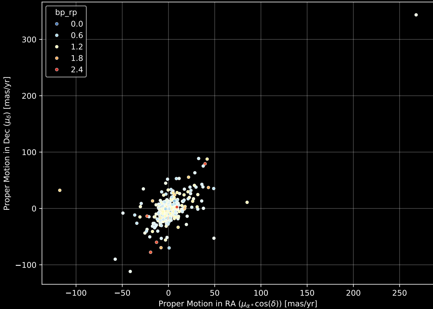
APOGEE DR17 Field: [K04_083+13] Proper Motion Diagram (n= 758)
