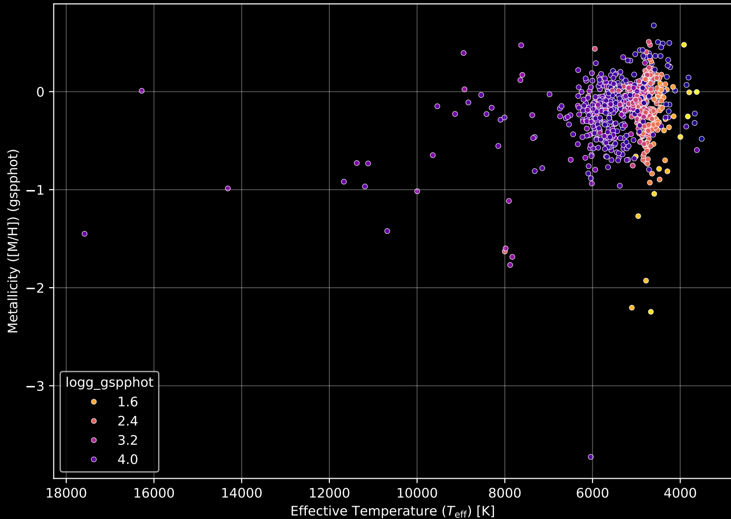
APOGEE DR17 Field: [K04_083+13] Stellar Population Parameters (n= 758)
